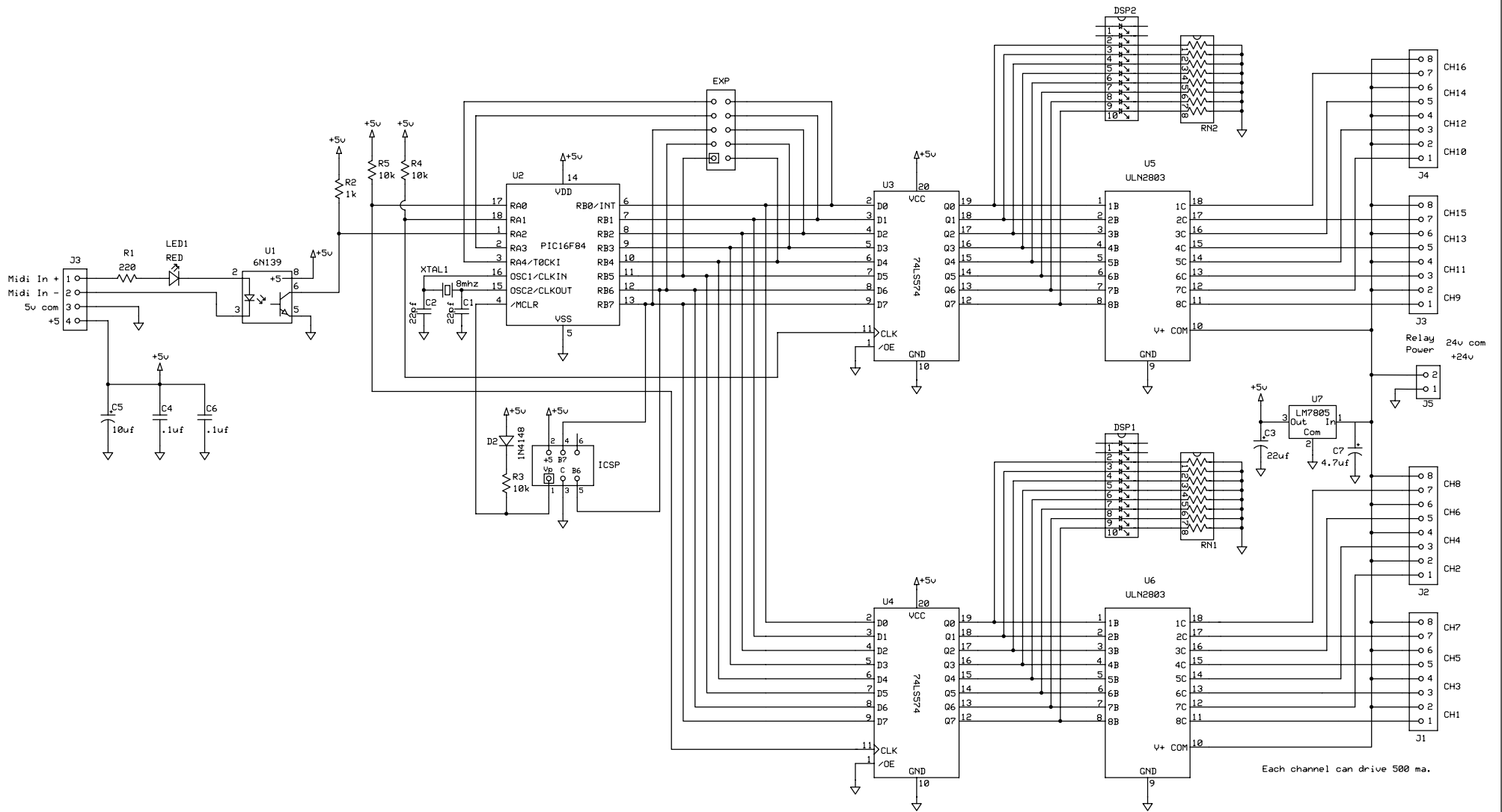
Botsmaker 16 channel Midi relay W. D. Sherman Rev 1.0 2/27/2010
